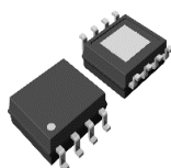
HSOP-8E 5.2 x 6.2 x 1.45 (mm)
