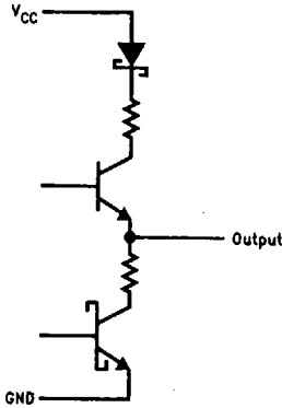
Schematic of Each Output
