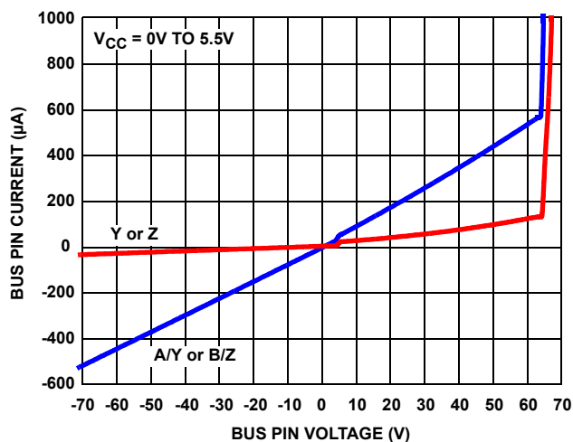
FIGURE 17. BUS PIN CURRENT vs BUS PIN VOLTAGE
