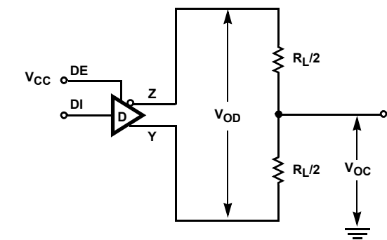
FIGURE 5A. V_{OD} AND V_{OC}
