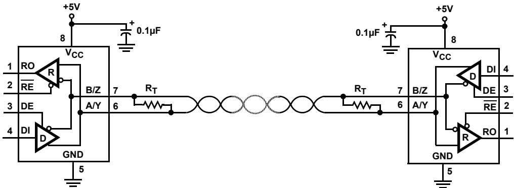
FIGURE 3. ISL32492E, ISL32495E, ISL32498E HALF DUPLEX EXAMPLE
