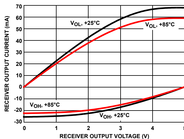
FIGURE 15. RECEIVER OUTPUT CURRENT vs RECEIVER OUTPUT VOLTAGE
