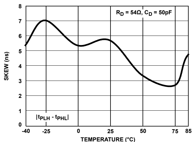
FIGURE 19. DRIVER DIFFERENTIAL SKEW vs TEMPERATURE (ISL32490E, ISL32492E)
