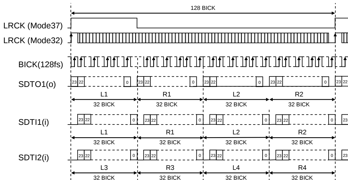
Figure 40. Mode 32/37 Timing (TDM128 Mode)
