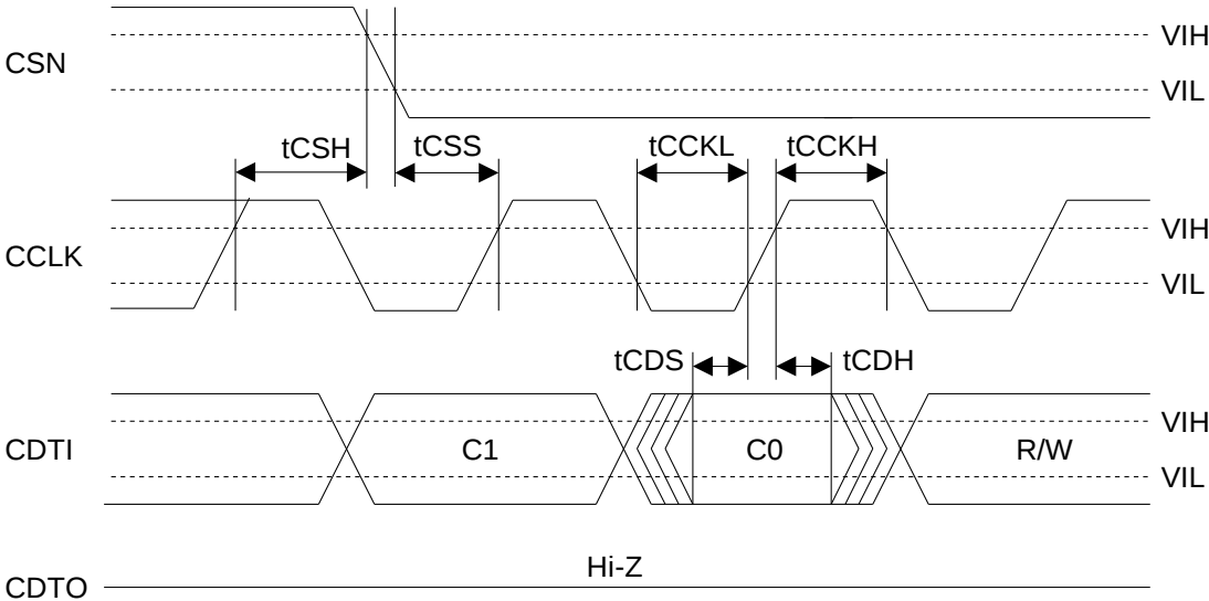
Figure 11. WRITE Command Input Timing (4-wire Serial mode)
