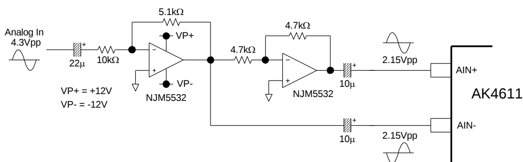
Figure 63. Input buffer circuit example 2 (AC coupled single-end input)
