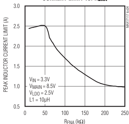
STEP-UP CONVERTER PEAK INDUCTOR CURRENT LIMIT vs. R_{ENA}
