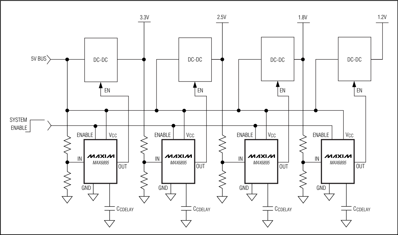
Figure 10. Multiple-Output Sequencing
