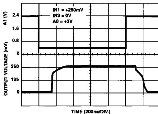
FIGURE 4. CHANNEL-TO-CHANNEL SWITCHING RESPONSE
