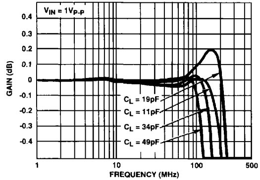
FIGURE 6. GAIN FLATNESS
