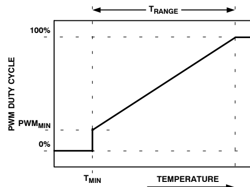
Figure 57. T RANGE Parameter Affects Cooling Slope
