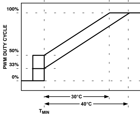
Figure 58. Adjusting PWM MIN Affects T_{\text{RANGE}}
