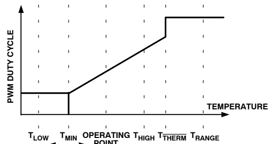
Figure 67. Dynamic T_{MIN} Control Loop
