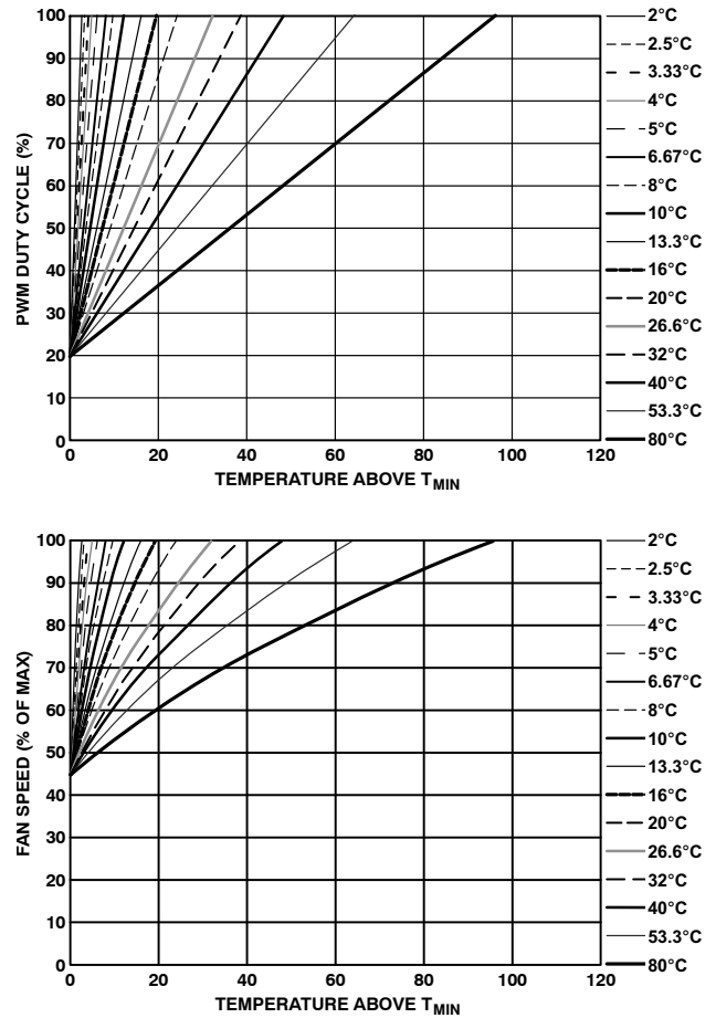
Figure 61. T_{\text{RANGE}} vs. % Fan Speed Slopes with \text{PWM}_{\text{MIN}} = 20\%
