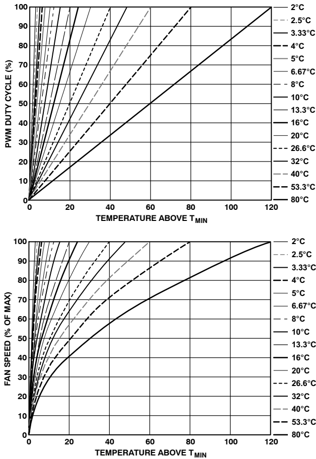
Figure 60. T_{\text{RANGE}} vs. Actual Fan Speed Profile
