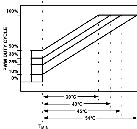
Figure 59. Increasing PWM MIN Changes Effective T_{\text{RANGE}}
