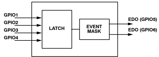
Figure 84. EDO Circuit
