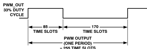
Figure 75. 33% PWM Duty Cycle Represented in Time Slots
