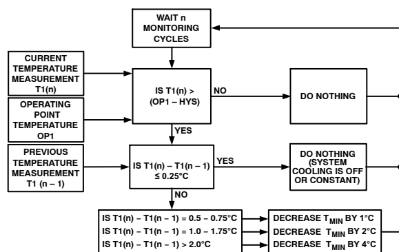
Figure 68. Short Cycle Steps
