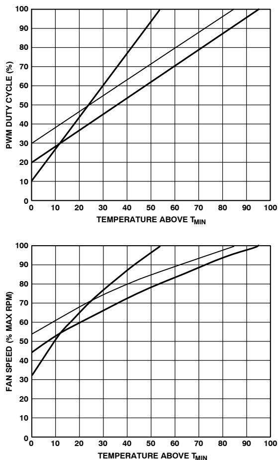
Figure 62. T_{\text{RANGE}} and % Fan Speed Slopes for VRM, Ambient, and CPU Temperature Channels
