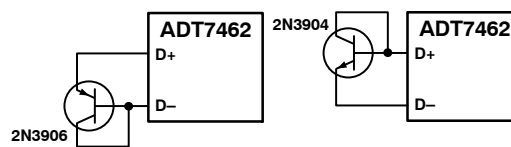
Figure 32. How to Measure Temperature Using Discrete Transistors
