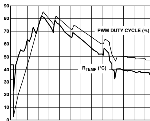
Figure 81. How Fan Reacts to Temperature Variations in Enhanced Acoustics Mode
