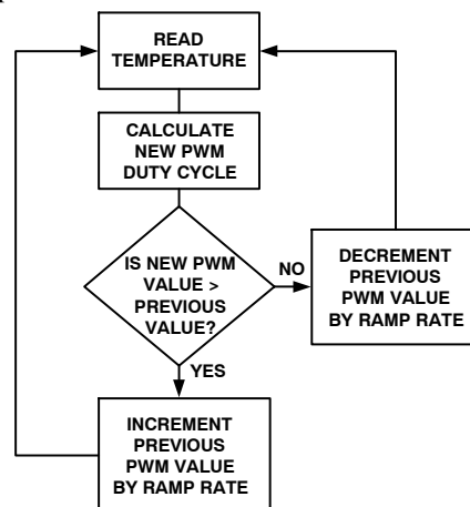
Figure 76. Enhanced Acoustics Mode Algorithm
