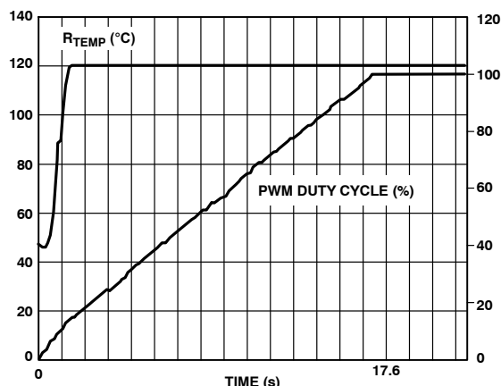
Figure 79. Enhanced Acoustics Mode with Ramp Rate = 2
