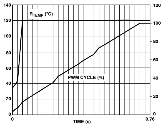
Figure 77. Enhanced Acoustics Mode with Ramp Rate = 48
