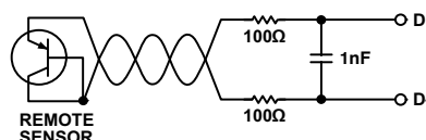
Figure 35. Filter Between Remote Sensor and ADT7462
