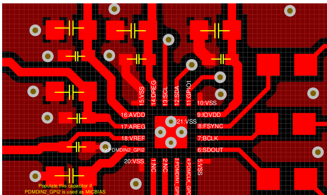
Figure 10-1. Layout Example
