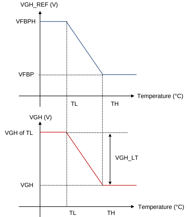
Figure 16. VGH Temperature Compensation Curve
