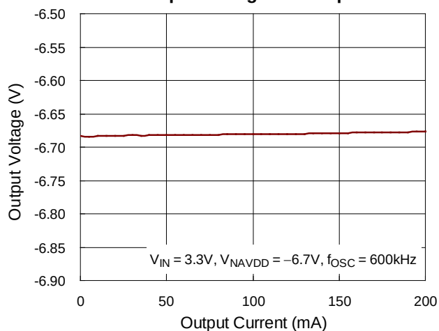
NAVDD Output Voltage vs. Output Current
