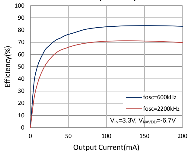
NAVDD Efficiency vs. Output Current
