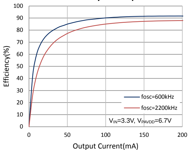
PAVDD Efficiency vs. Output Current
