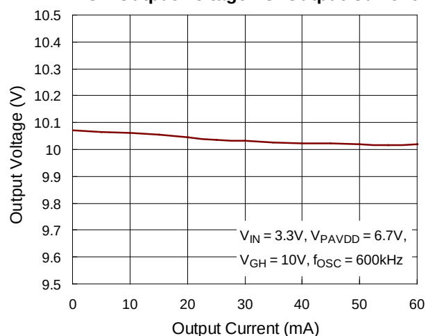
VGH Output Voltage vs. Output Current
