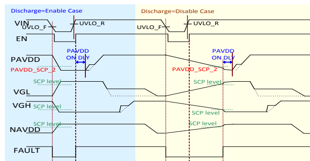
Figure 10. The Power-up Limitation of The Outputs Voltage must below the SCP level
