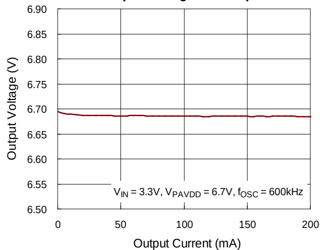
PAVDD Output Voltage vs. Output Current
