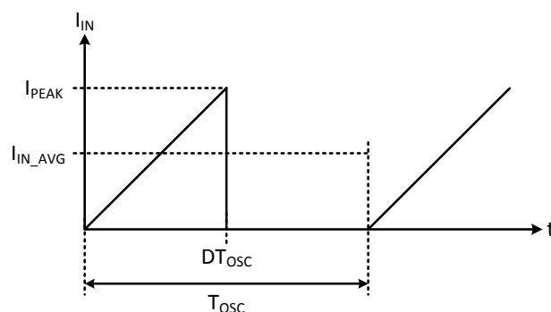
Figure 17. The Buck-boost Input Signature in BCM
