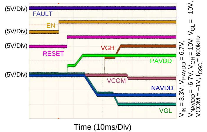
Power On
