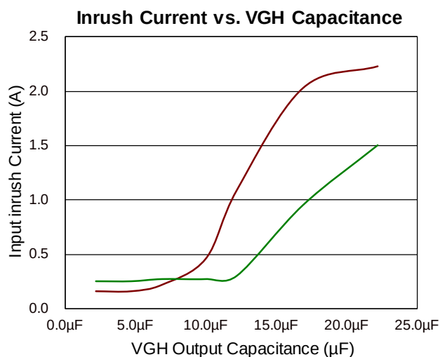
Figure 14. Inrush current vs. VGH capacitance
