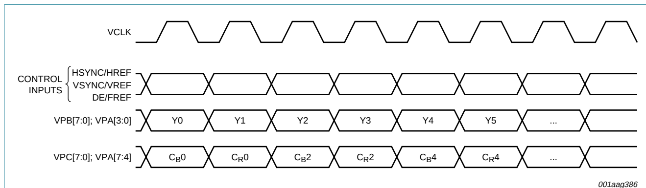
Fig 9. Pixel encoding YC B C R 4 : 2 : 2 semi-planar external synchronization (rising edge) input
