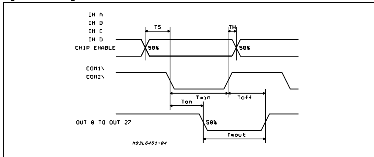
Figure 3. Timing waveforms
