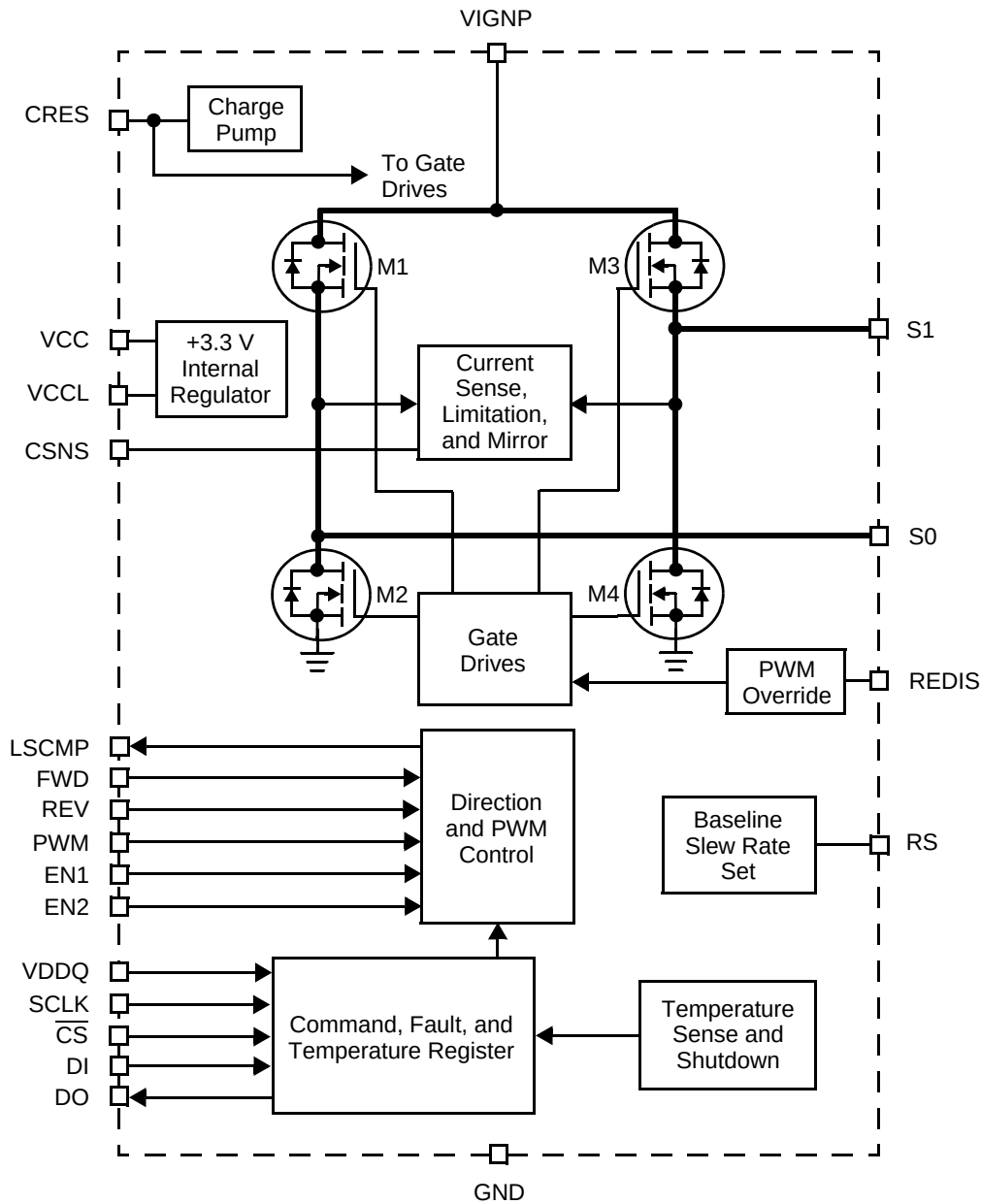
Figure 2. 33899 Simplified Internal Block Diagram
