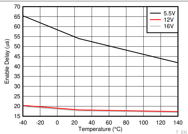
Figure 6-12. Enable Delay
