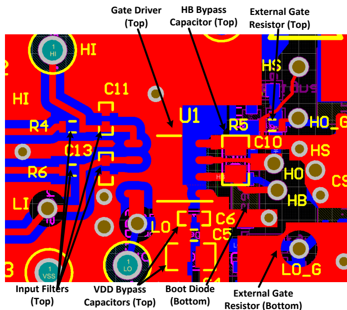
Figure 10-1. Layout Example
