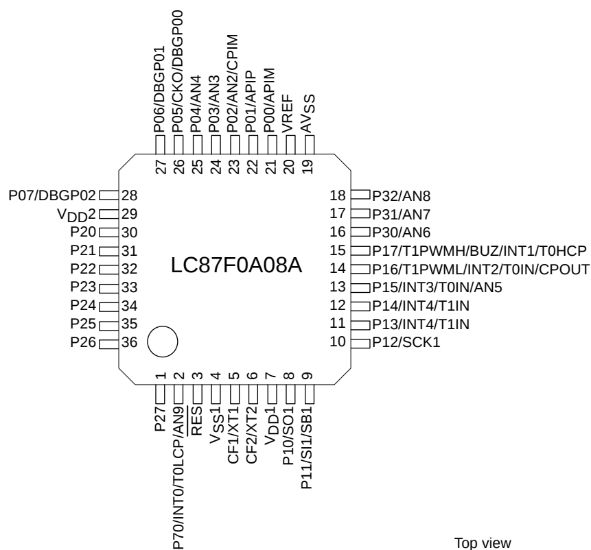
Top view
