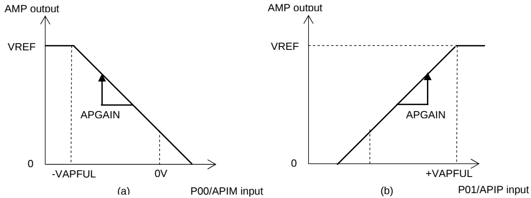
Figure 7 20× Amplifier Characteristics
