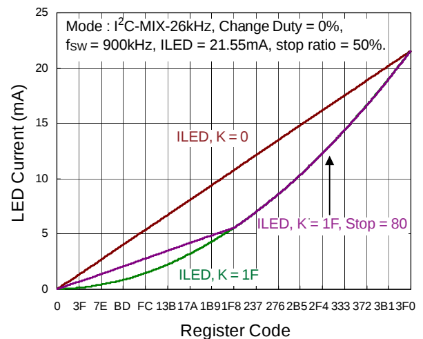
Figure 5. LED Current vs. Register Code
