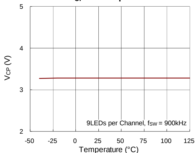
V_{CP} vs. Temperature
