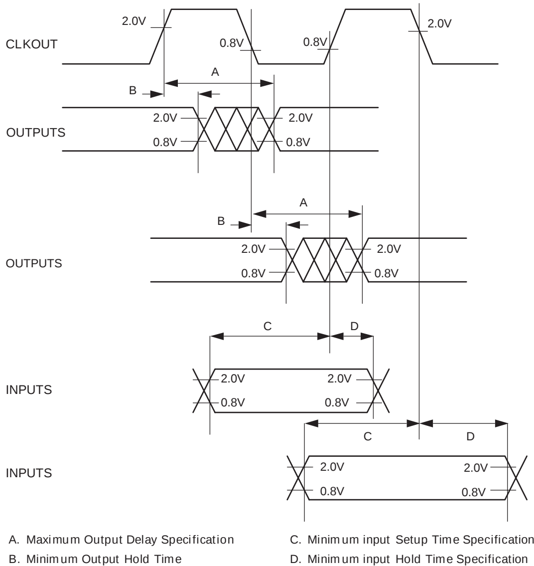
Figure 7. AC Electrical Specifications Control Timing Diagram
