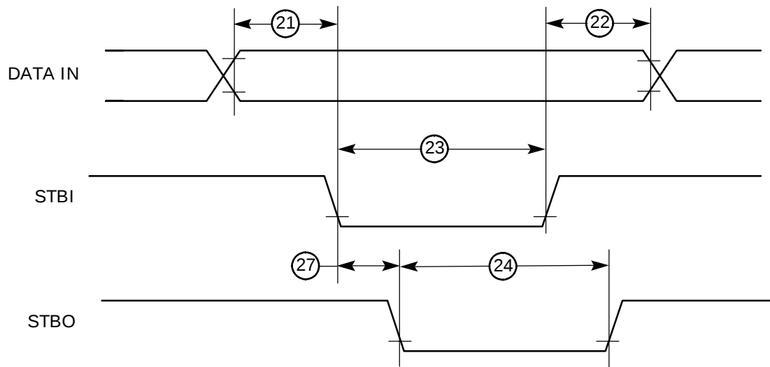
Figure 43. PIP RX (Interlock Mode) Timing Diagram
