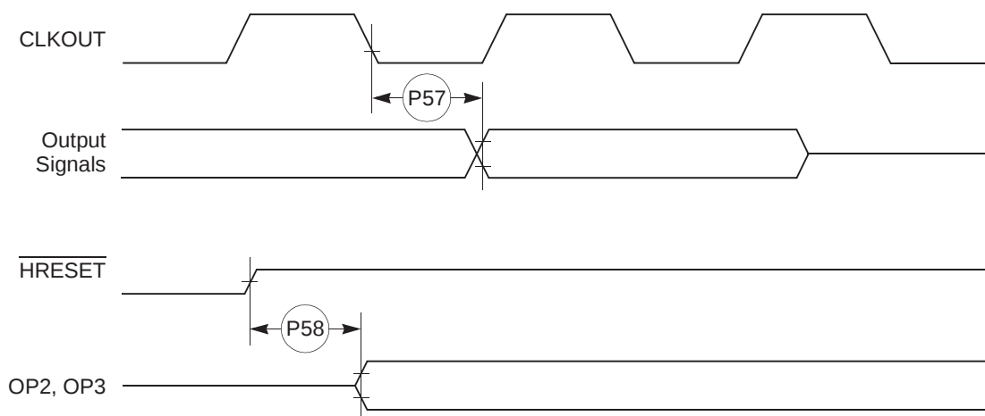
Figure 32. PCMCIA Output Port Timing
