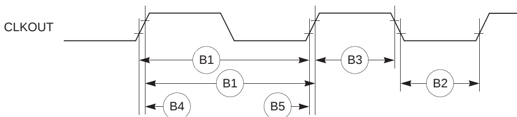
Figure 8. External Clock Timing
