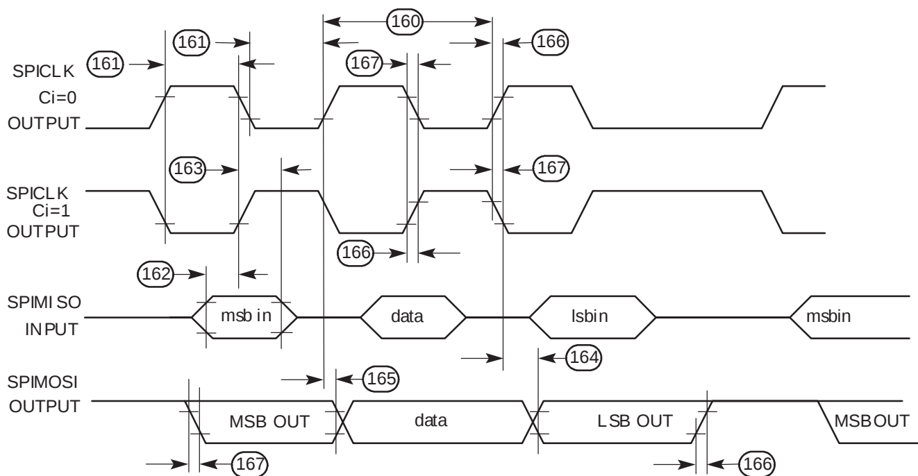
Figure 69. SPI Master (CP = 1) Timing Diagram
