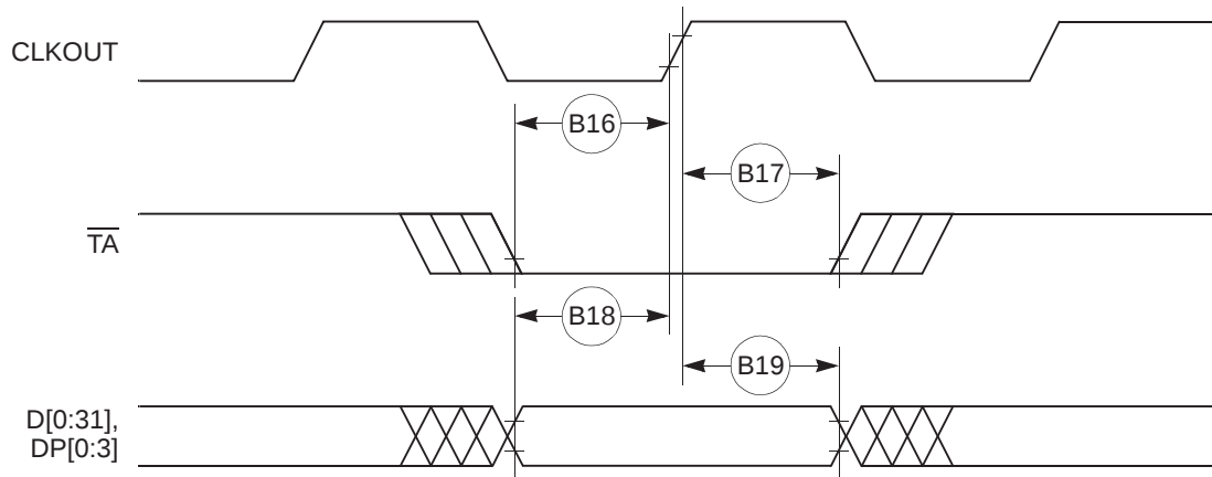
Figure 12. Input Data Timing in Normal Case
