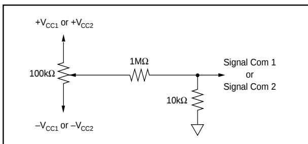
FIGURE 3. V_{OS} Adjust.
