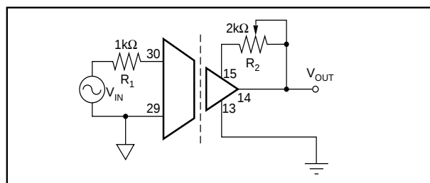
FIGURE 2a. Gain Adjust.
