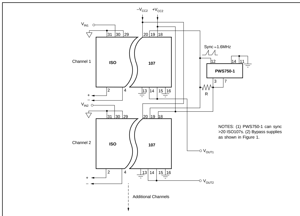
FIGURE 6. Synchronized-Multichannel Isolation.
