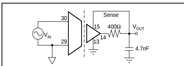
FIGURE 4. Ripple Reduction.
