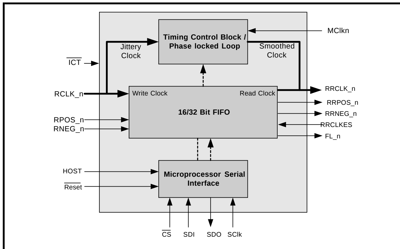
FIGURE 6. A TYPICAL CHANNEL_N OF THE XRT71D04 CONFIGURED TO OPERATE IN THE HOST MODE
