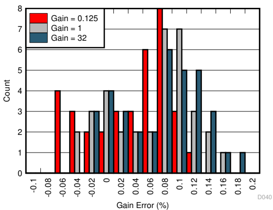
Figure 7-18. Gain Error Distribution
