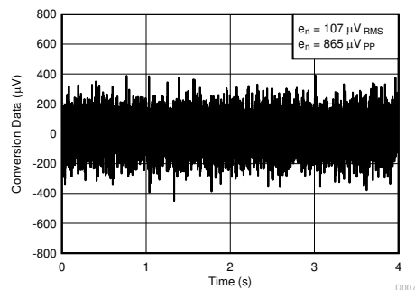
Figure 10-2. Conversion Noise
