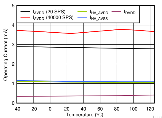
Figure 7-30. Operating Current vs Temperature
