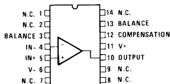
HA1-2542 (CERAMIC DIP) HA3-2542 (PLASTIC DIP) TOP VIEW
