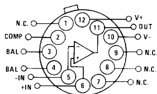
HA2-2542 (TO-8 METAL CAN) TOP VIEW
