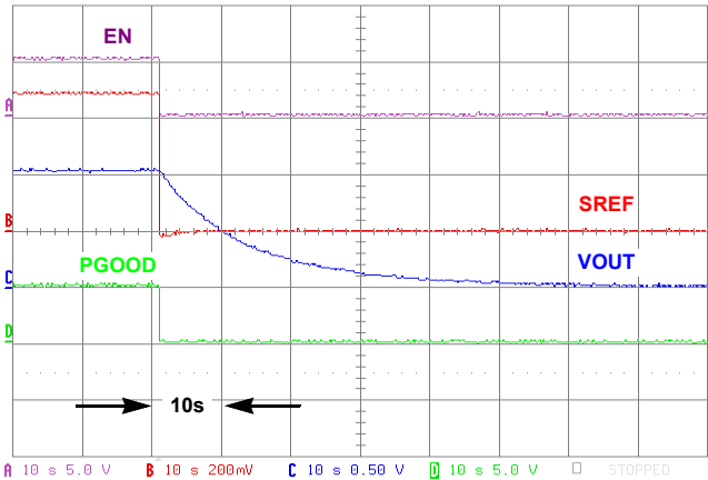
FIGURE 19. SHUT-DOWN, V_{IN} = 12.6V , V_{OUT} = 1.05V , I_{LOAD} = \text{OPEN-CIRCUIT}
