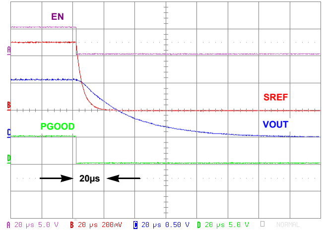
FIGURE 18. SHUT-DOWN, V_{IN} = 12.6V , V_{OUT} = 1.05V , I_{LOAD} = 50m\Omega
