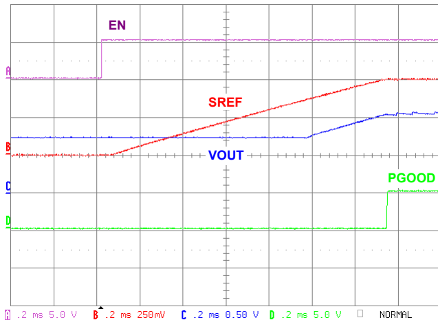
FIGURE 17. START-UP INTO 750mV PRE-BIASED OUTPUT, V_{IN} = 12.6V , V_{OUT} = 1.05V , I_{LOAD} = 10A
