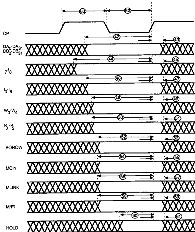
Setup and Hold Timing
