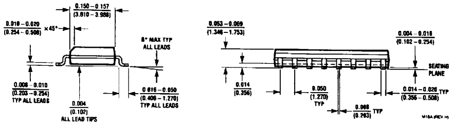
16-Lead Small Outline Molded Package (M) Order Number DM74LS366AM NS Package Number M16A
