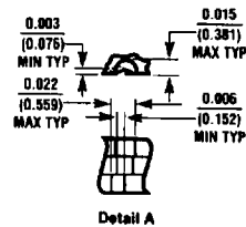
Ceramic Leadless Chip Carrier Package (E) Order Number DM54LS366AE NS Package Number E20A
