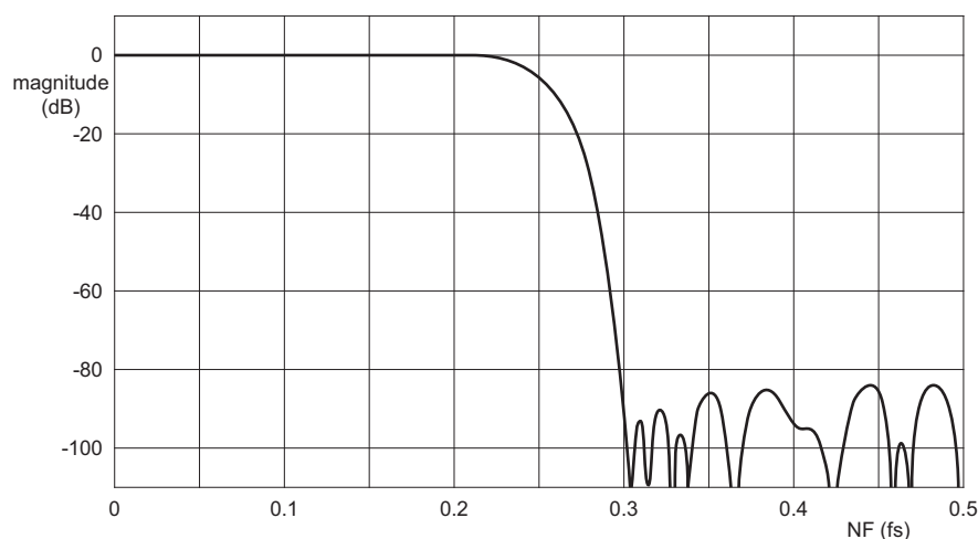
Fig 30. First stage half-band filter response
