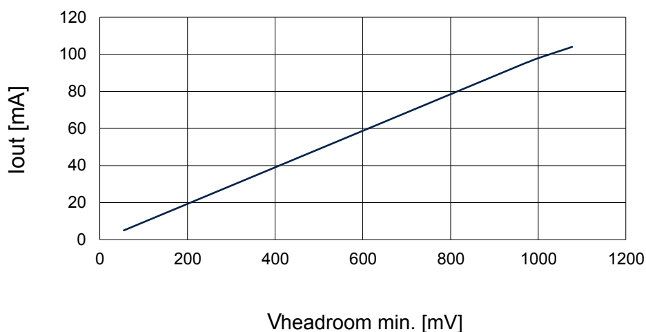
Figure 7. Minimum V_{headroom} vs. I_{OUT} ( T_J = 25\text{ °C} )
