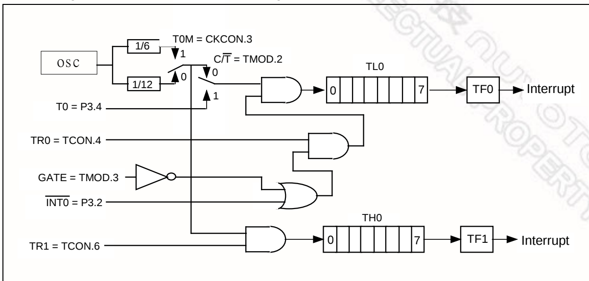
Figure 9-3 Timer/Counter 0 Mode 3
