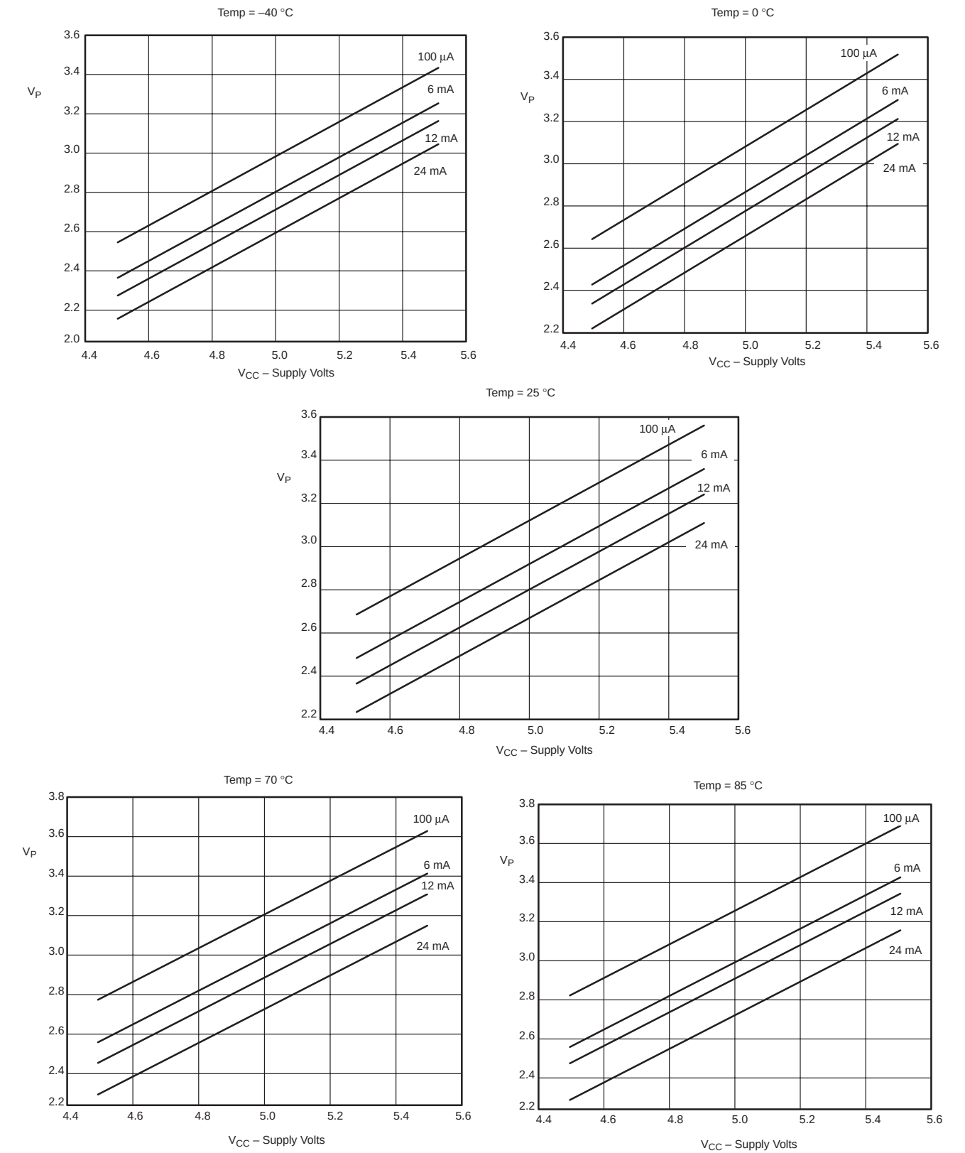
Figure 1. Typical characteristics
