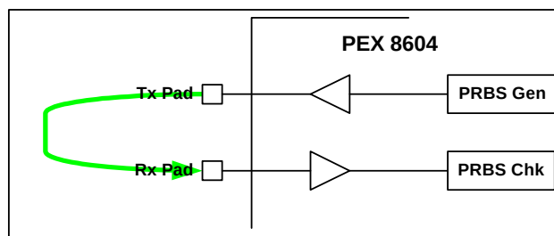
Figure 18-2. Cable Loopback
