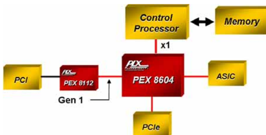
Figure 2-2. Fan-In/Fan-Out Usage
