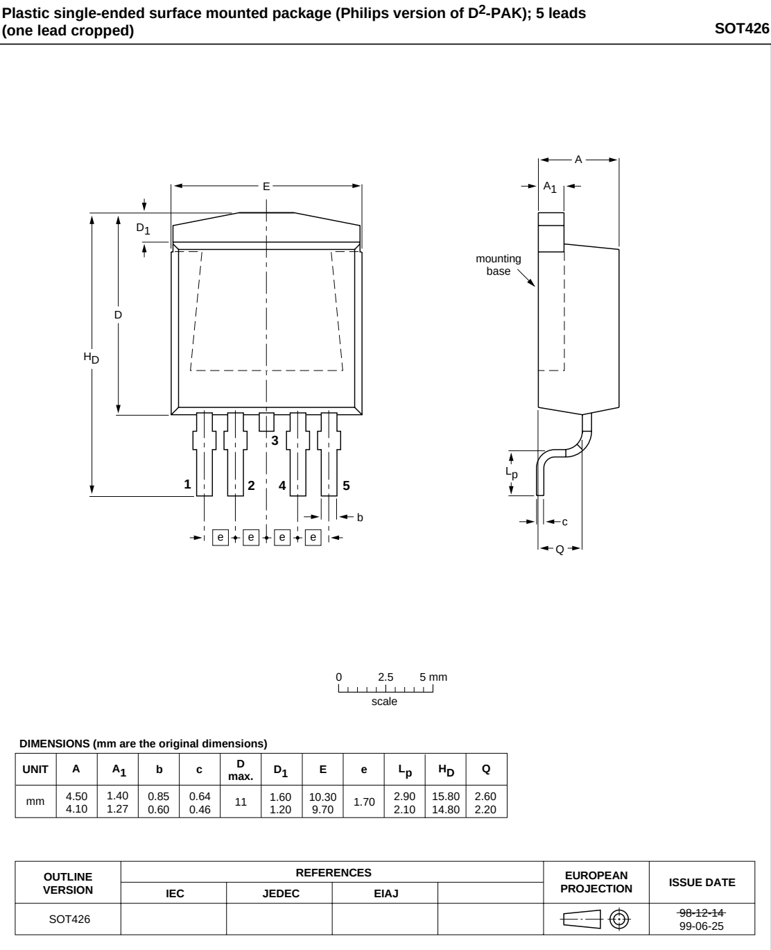
Fig.36. SOT426 surface mounting package 1 , centre pin connected to mounting base.
