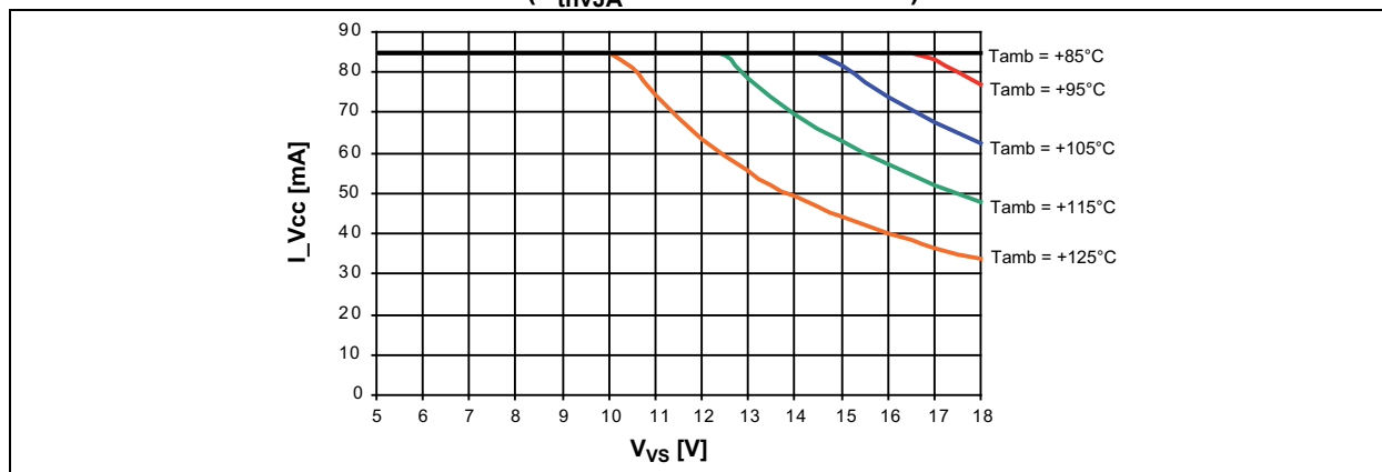
FIGURE 1-13: POWER DISSIPATION: SAFE OPERATING AREA: REGULATOR'S OUTPUT CURRENT I_{VCC} VERSUS SUPPLY VOLTAGE V_{VS} AT DIFFERENT AMBIENT TEMPERATURES ( R_{thJA} = 45 K/W ASSUMED)
