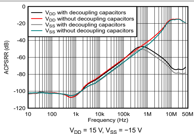
Figure 6-28. ACPSRR vs Frequency
