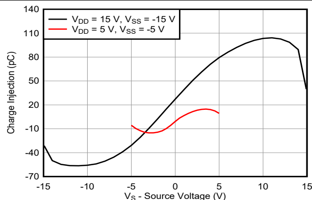
Figure 6-13. Charge Injection vs Source Voltage – Dual Supply
