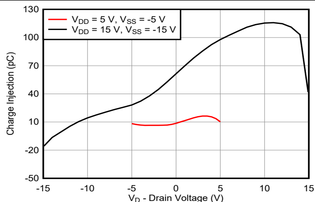
Figure 6-14. Charge Injection vs Drain Voltage – Dual Supply
