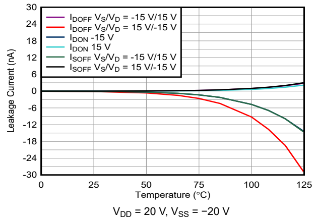
Figure 6-8. On-Leakage vs Temperature
