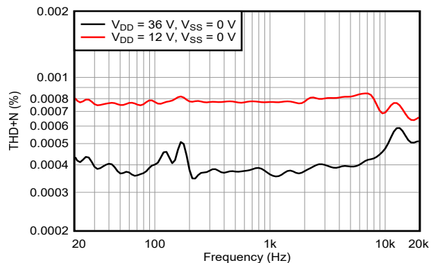
Figure 6-26. THD+N vs Frequency – Single Supply
