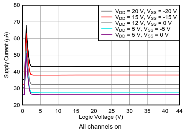
Figure 6-12. Supply Current vs Logic Voltage
