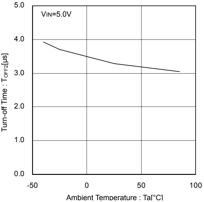
Figure 27. Output Turn-off Time vs Ambient Temperature
