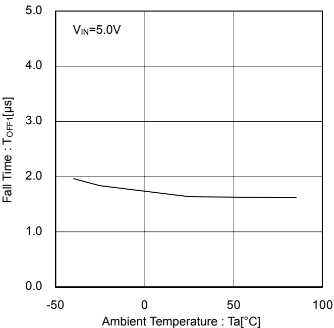
Figure 25. Output Fall Time vs Ambient Temperature
