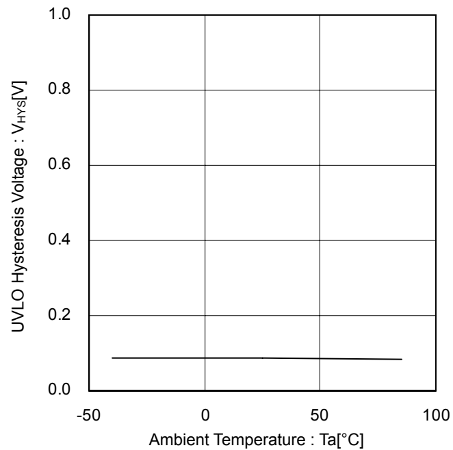
Figure 19. UVLO Hysteresis Voltage vs Ambient Temperature
