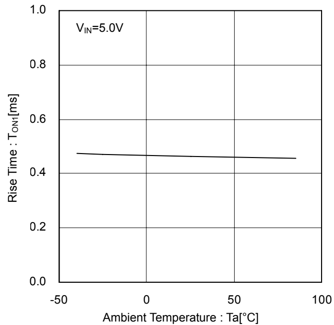
Figure 21. Output Rise Time vs Ambient Temperature
