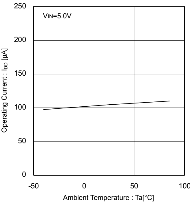
Figure 7. Operating Current vs Ambient Temperature EN Enable
