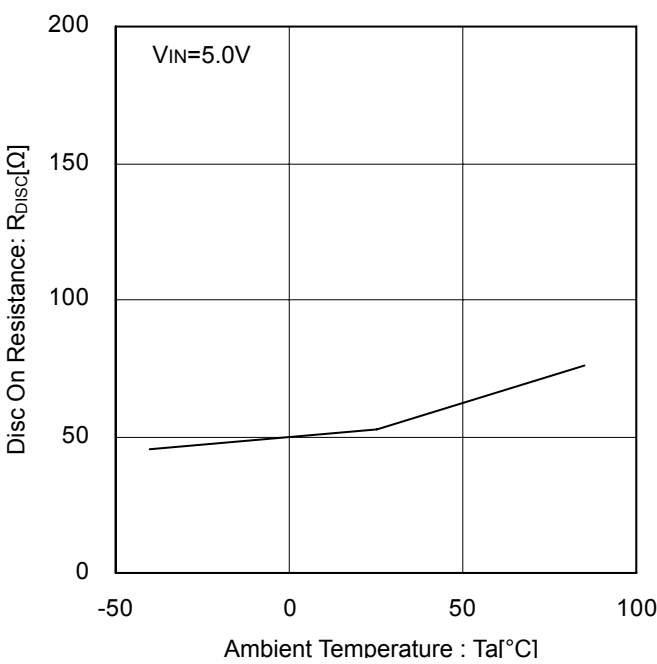
Figure 31. Discharge On Resistance vs Ambient Temperature
