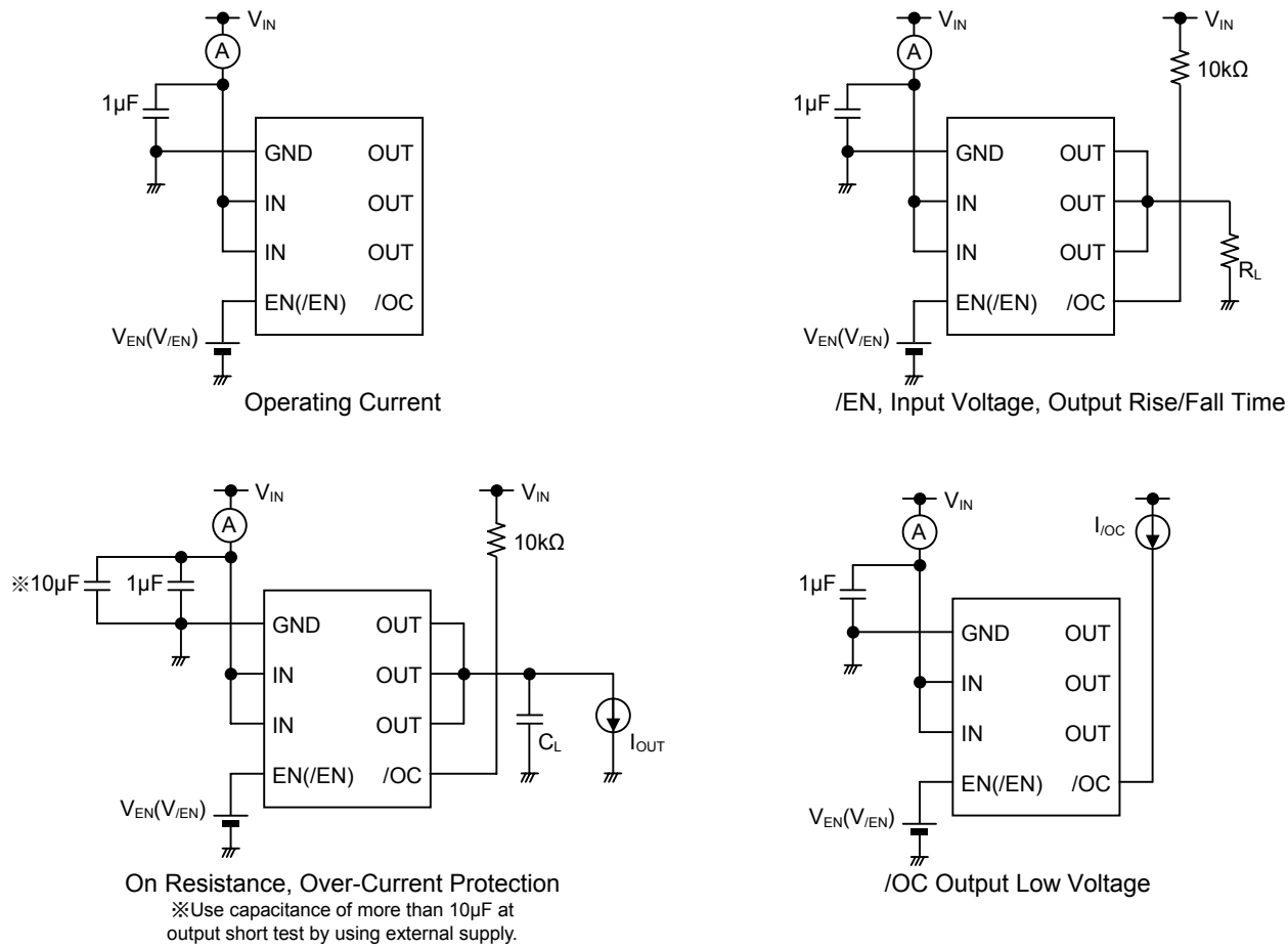
Figure 4. Measurement Circuit
