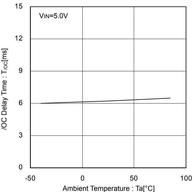
Figure 29. /OC Delay Time vs Ambient Temperature
