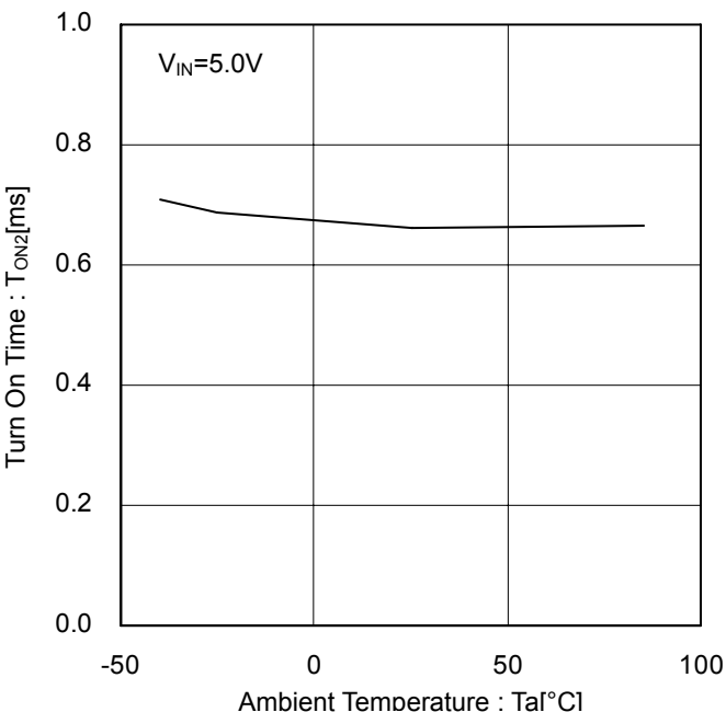
Figure 23. Output Turn-on Time vs Ambient Temperature
