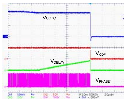
Figure 10: Over-Current Latch-off Waveforms
