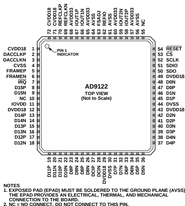
Figure 4. Pin Configuration
