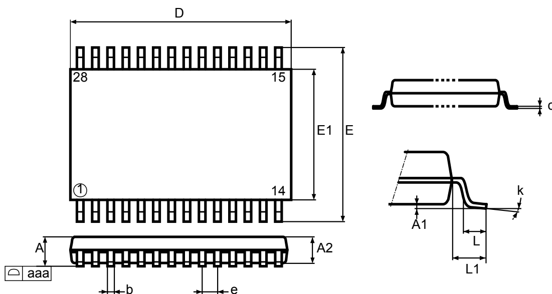
Figure 5. TSSOP28 - outline
