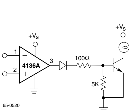
Figure 21. Lamp Driver
