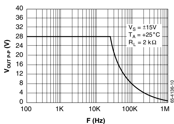
Figure 8. Output Voltage Swing vs. Frequency
