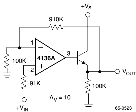
Figure 22. Power Amplifier
