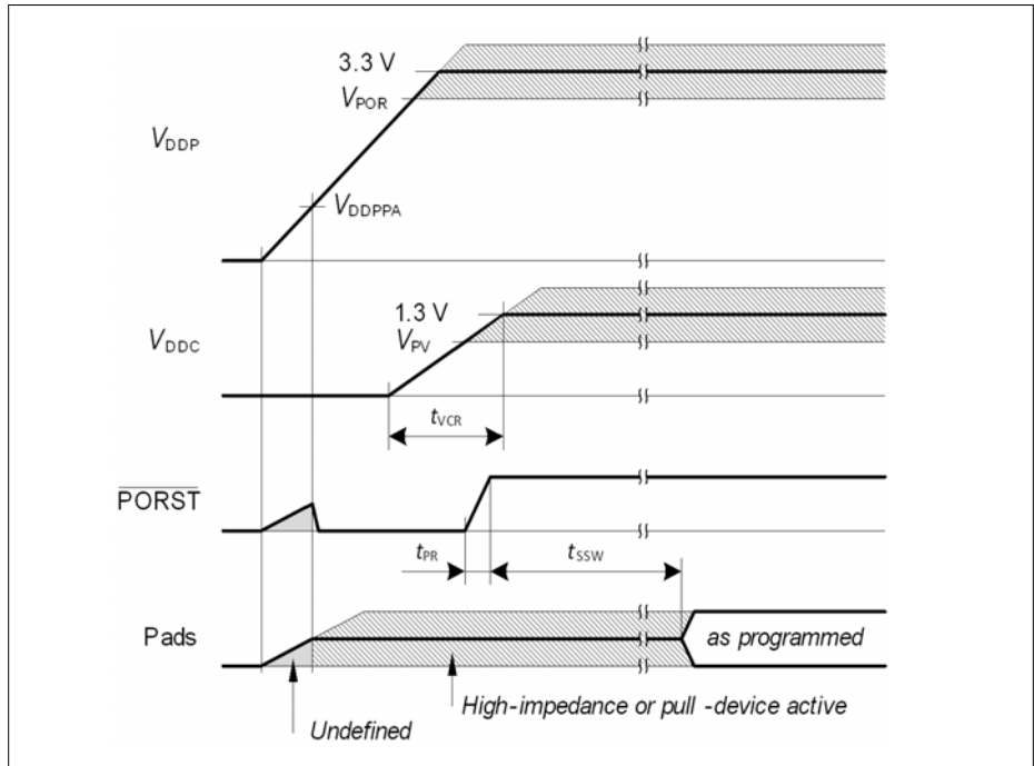
Figure 26 Power-Up Behavior
