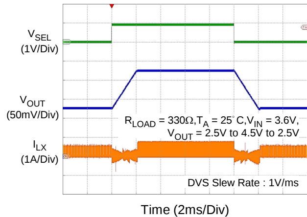
Dynamic Voltage Scaling (RPWM Function Enable)
