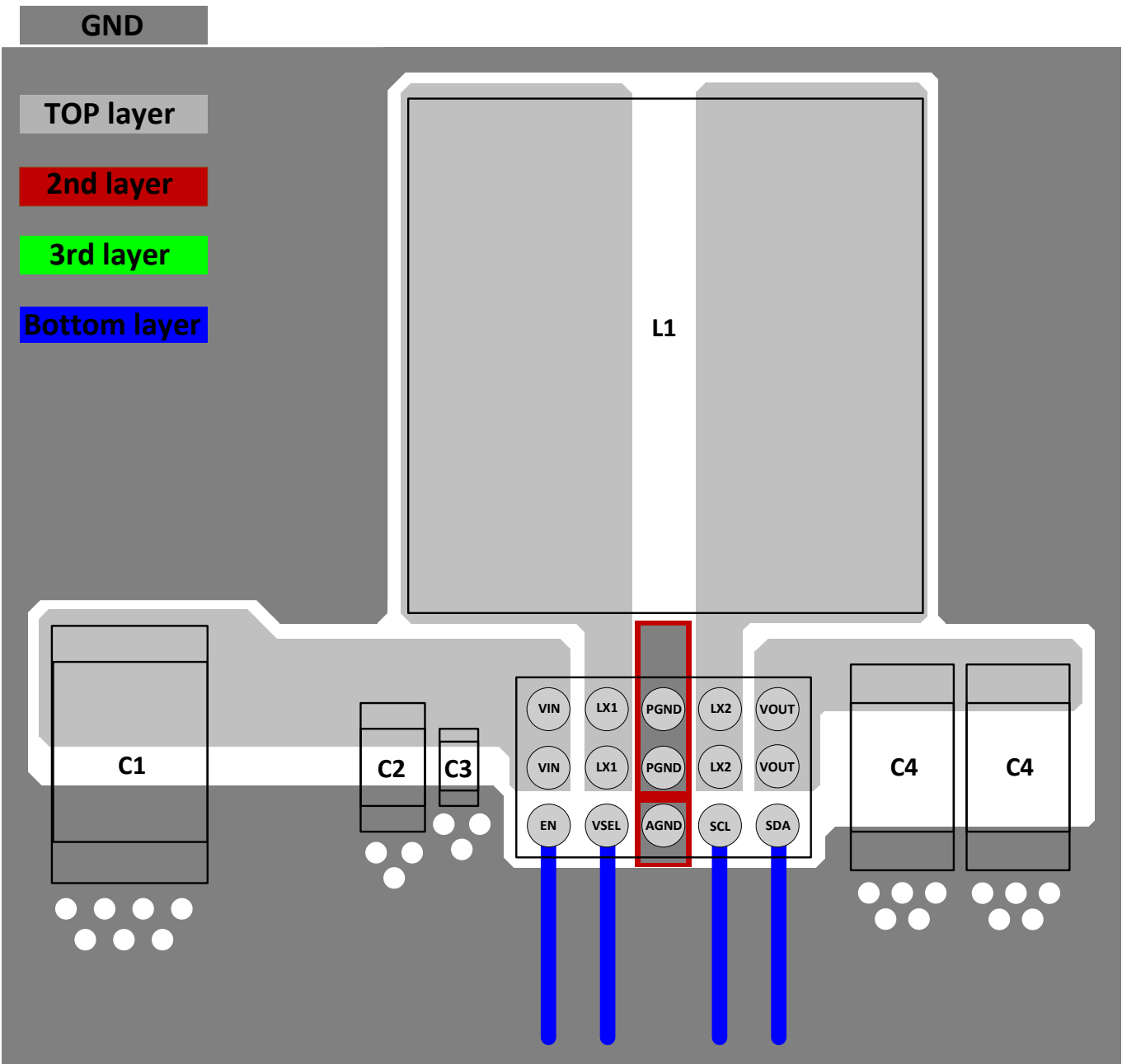
Figure 7. Layout Guide
