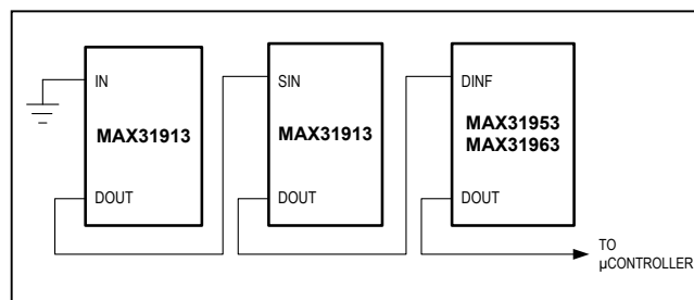
Figure 8. Daisy Chaining
