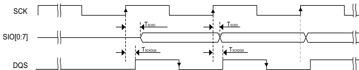
Figure 21. FlexSPI input timing in SDR mode where FlexSPI_MCR0[RXCLKSRC] = 0X3 (Case A1)
