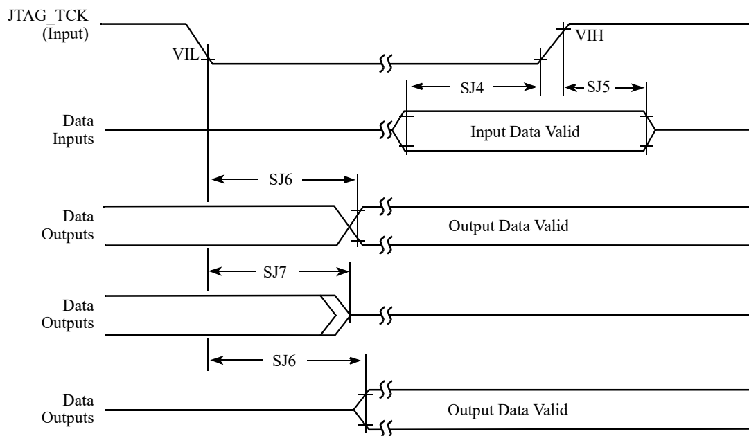
Figure 11. Boundary scan (JTAG) timing diagram
