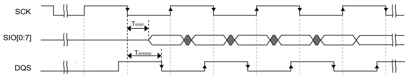
Figure 24. FlexSPI input timing in DDR mode where FlexSPIn_MCR0[RXCLKSRC] = 0x3 (Case B1)
