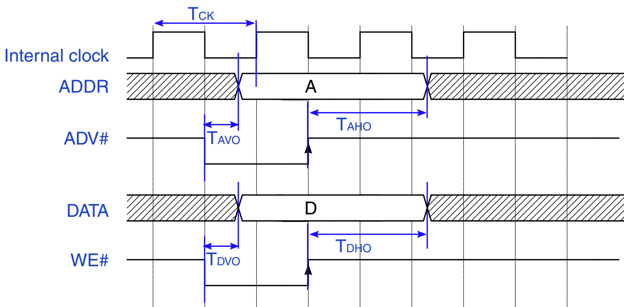
Figure 16. SEMC output timing in ASYNC mode
