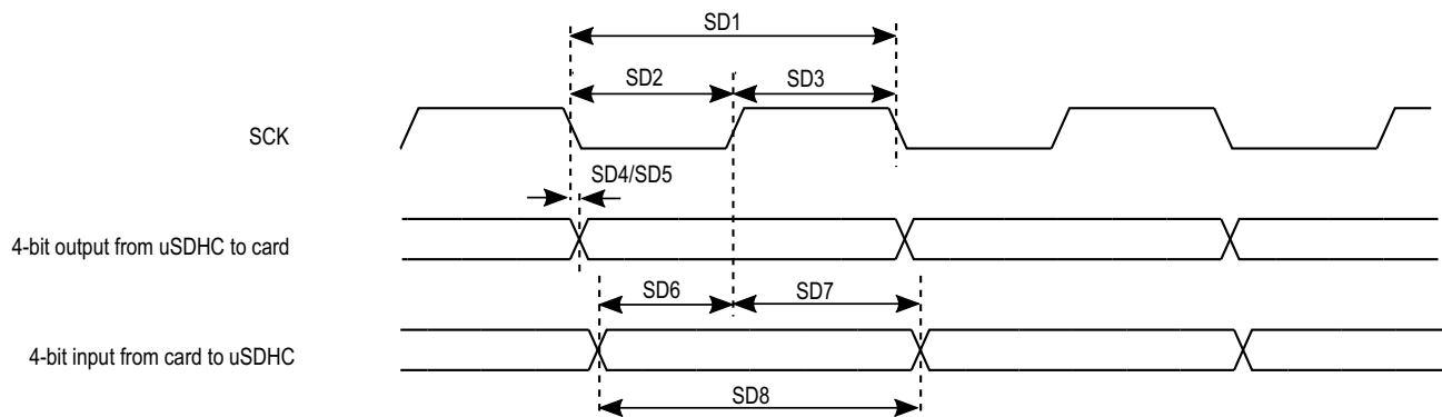
Figure 42. SDR50/SDR104 timing
