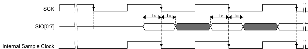
Figure 20. FlexSPI input timing in SDR mode where FlexSPI_MCR0[RXCLKSRC] = 0X0, 0X1
