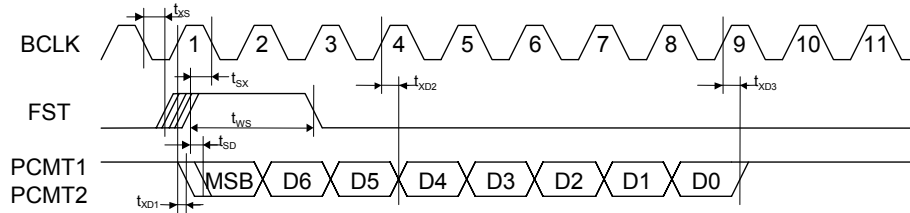
Figure 8-5a. Transmit Timing
