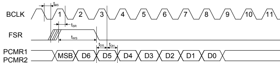
Figure 8-5b. Receive Timing
