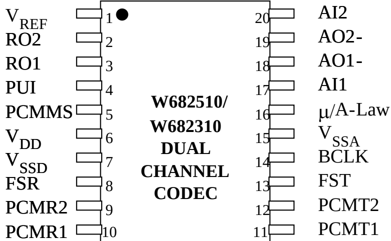
PDIP (W682510 only), SSOP
