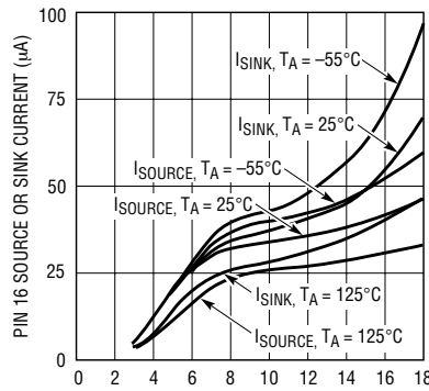
C_{osc} Pin I_{SINK} , I_{SOURCE} vs Supply Voltage
