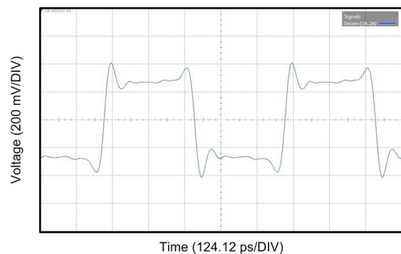
Figure 21. DS280DF810 FIR Transmit Equalization while Operating at 25.78125 Gbps
