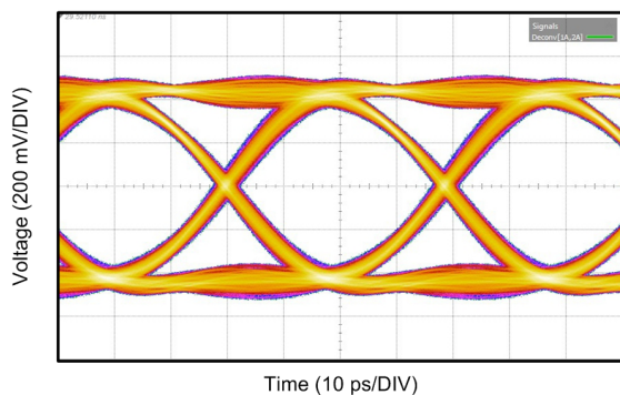
Figure 20. DS280DF810 Operating at 25.78125 Gbps
