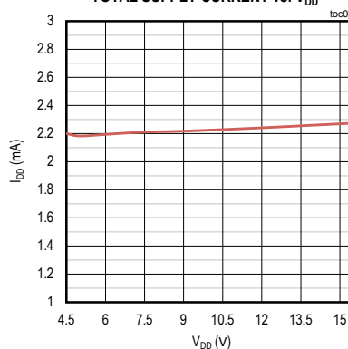
TOTAL SUPPLY CURRENT vs. V_{DD}
