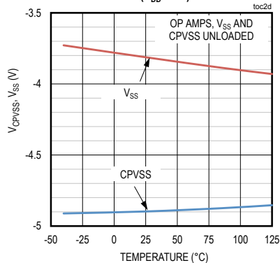
CPVSS AND V_{SS} vs. TEMPERATURE ( V_{DD} = 5\text{V} )
