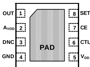
ISL24202 (8 LD TDFN) TOP VIEW
