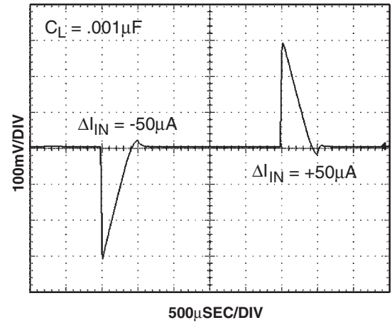
50μA LOAD TRANSIENT RESPONSE
