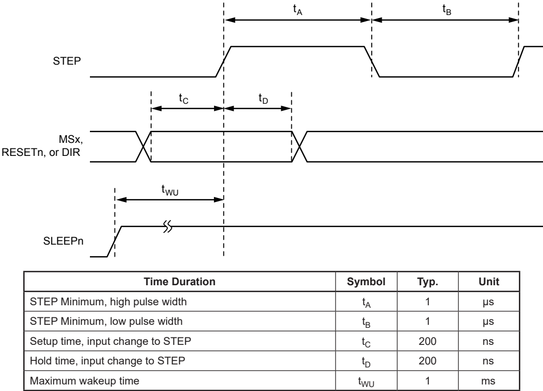
Figure 1: Logic Interface Timing Diagram
