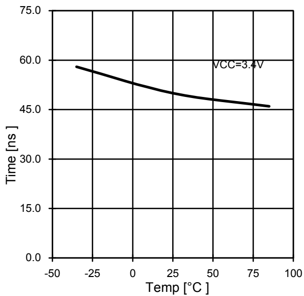
Fig.26 IGBT Response time Fall1 (START=0)
