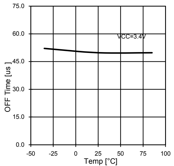
Fig.19 MAX OFF Time
