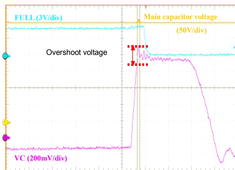
Fig36.Waveform of VC pin overshoot voltage
