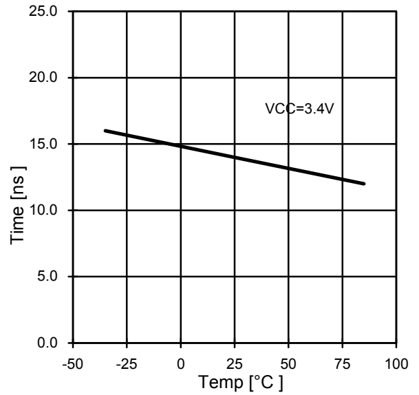
Fig.25 IGBT Response time Rise1 (START=0)
