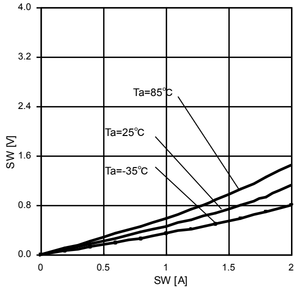
Fig.16 SAT Voltage
