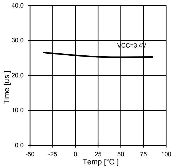
Fig.18 START Delay Time
