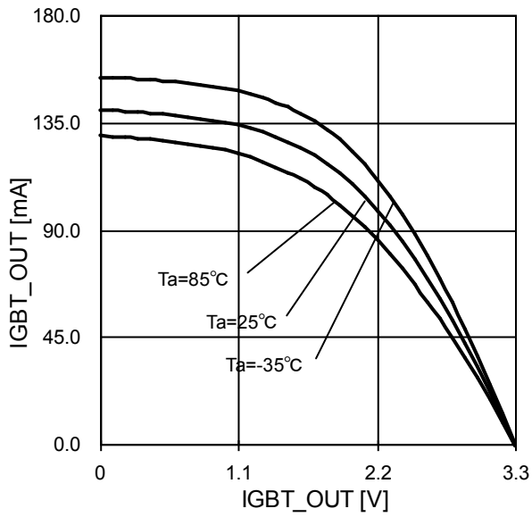
Fig.24 IGBT_OUT Source Current
