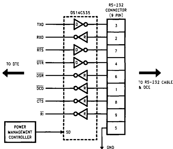
FIGURE 9. Typical DTE Application
